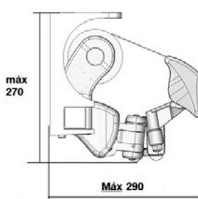
SOPORTE MONOBLOC EPSYLON MONOBLOC EPSYLON SUPPORT
