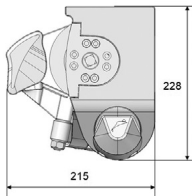
SOPORTE EPSYLON EPSYLON SUPPORT SUPPORT EPSYLON SUPORTE EPSILON
