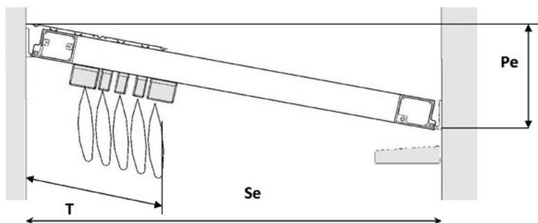
Ref. 106199_ Soporte Guía 80x40 Extrusión Aluminio Extruded aluminium guide support 80 x 40 Support Rail de guidage 80x40 Extrusion Aluminium Suporte Guia 80x40 Extrusão Alumínio
