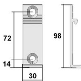
SOPORTE COFRE VERTICAL 110/125 VERTICAL COFFER SUPPORT 110/125 SUPPORT COFRE VERTICAL 110/125 SUPORTE COFRE VERTICAL 110/125
