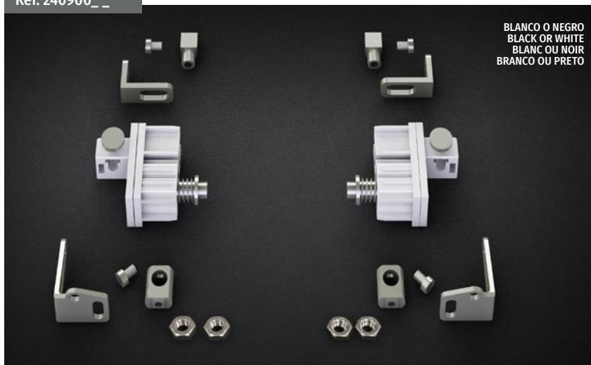
Kit tordo vertical cable / Cable-guided system kit / Kit store vertical guidé par câble / Kit tordo vertical cabo
