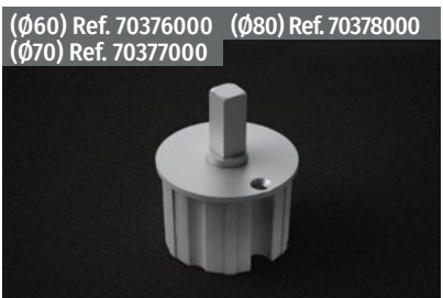
Casquillo máquina nylon Nylon machine Valve Holder Douille machine nylon Casquilho máquina nylon
