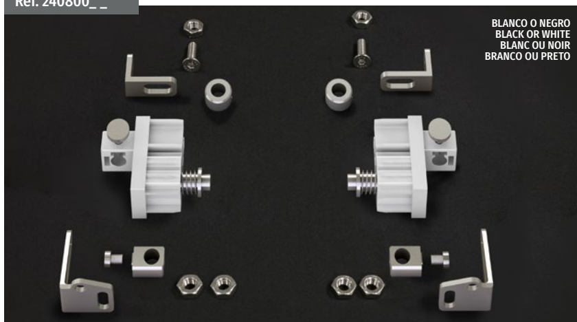
Kit tordo vertical varilla / Rod-guided system kit / Kit store vertical guidé par tige / Kit tordo vertical vareta
